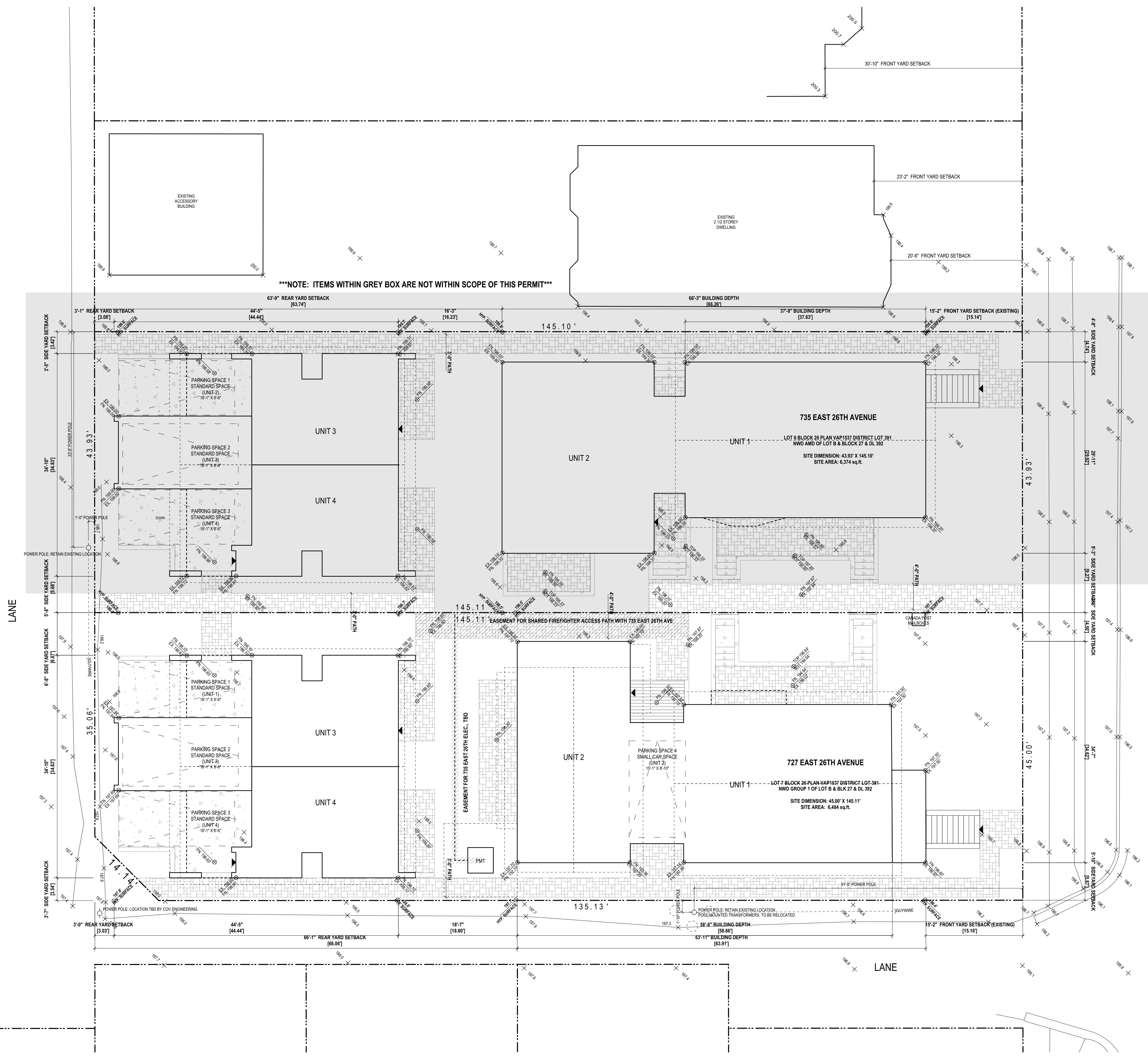
1 SITE PLAN 1/8" = 1'-0"
