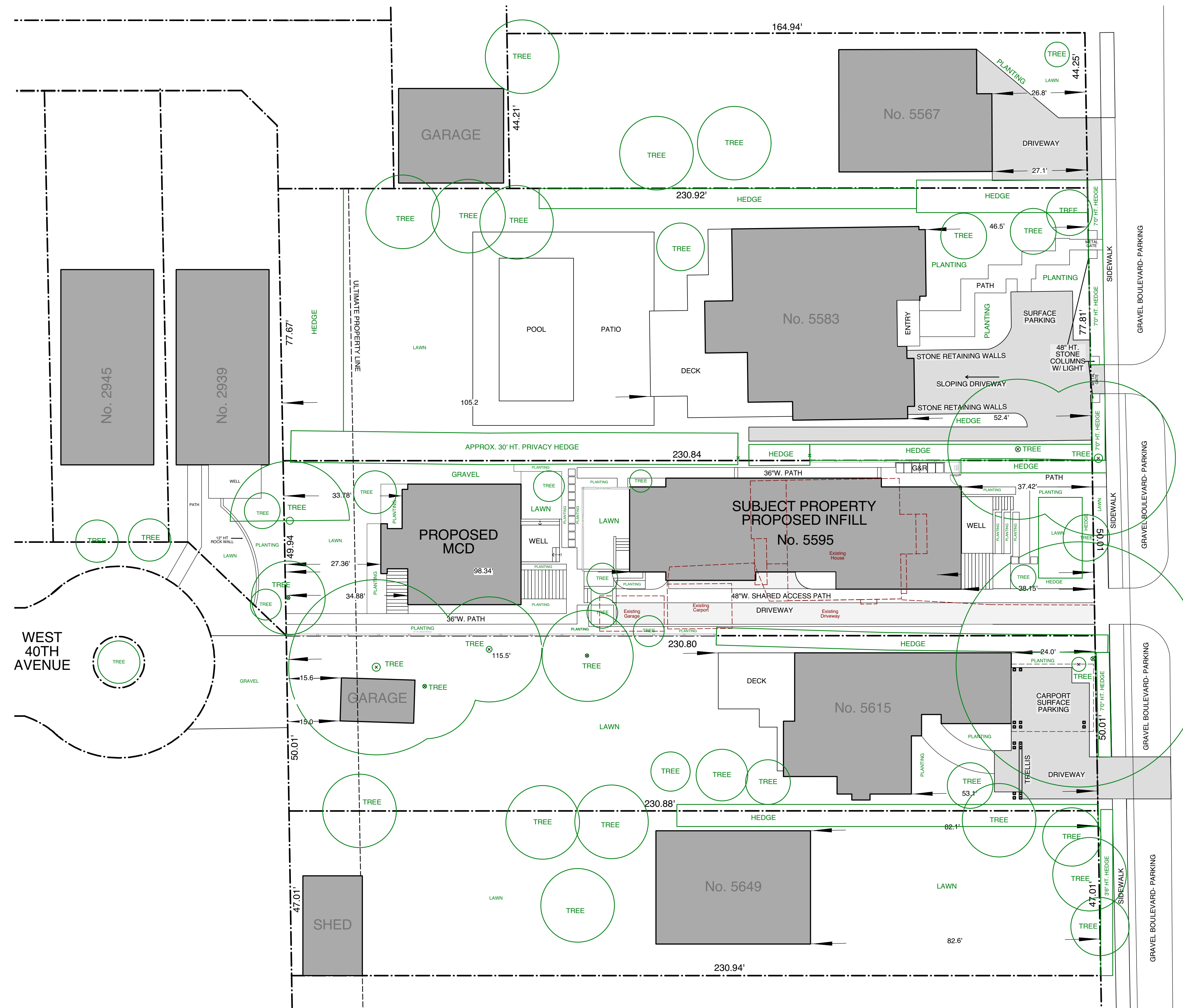
3 NEIGHBOURHOOD SITE CONTEXT PLAN Scale: 1/16" = 1'-0"
