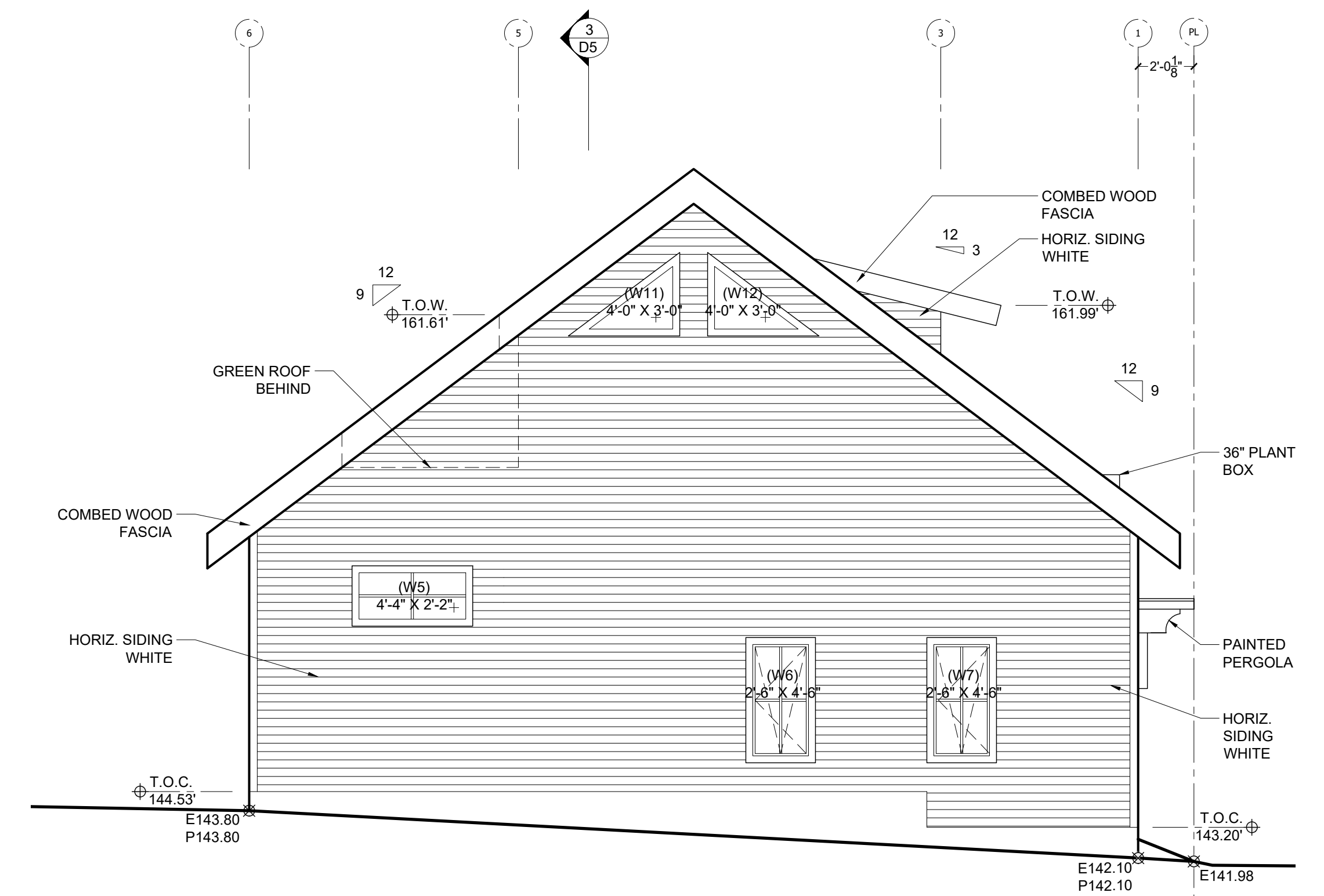
D5.1-3 PROPOSED INFILL - EAST ELEVATION 1/4" - 1'-0"
