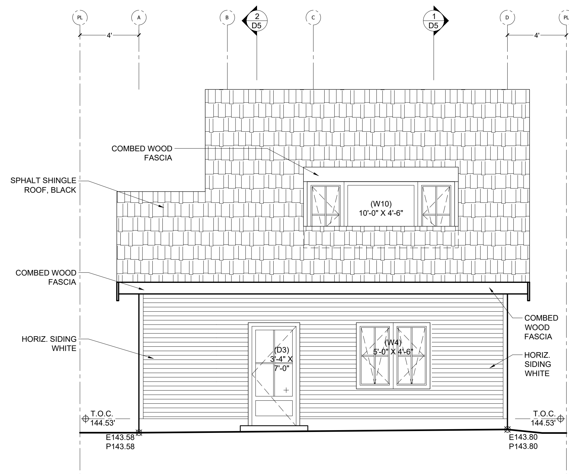
D5.1-2 PROPOSED INFILL - SOUTH ELEVATION 1/4" - 1'-0"
