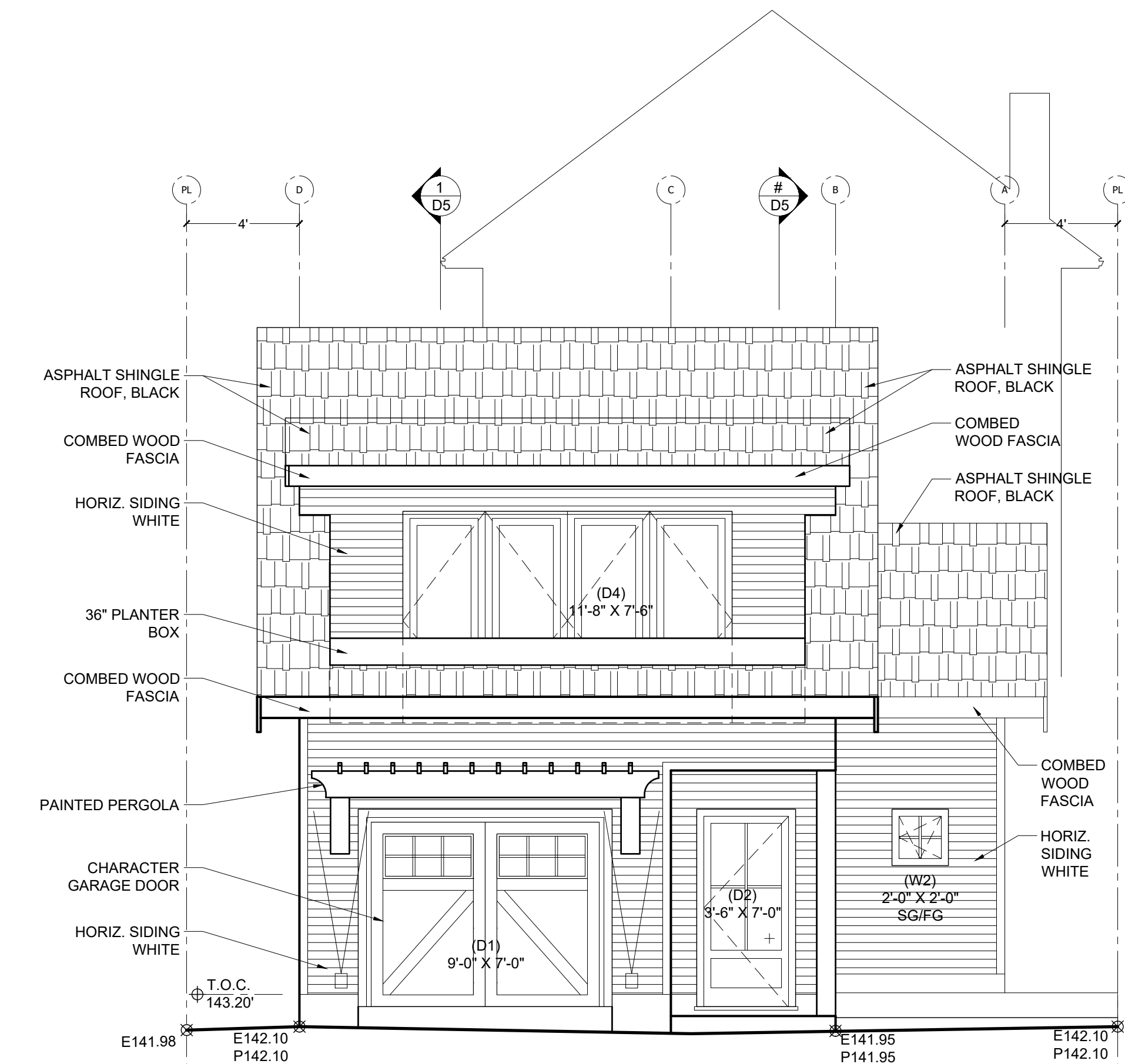
D5.1-1 PROPOSED INFILL - NORTH ELEVATION 1/4" - 1'-0"
