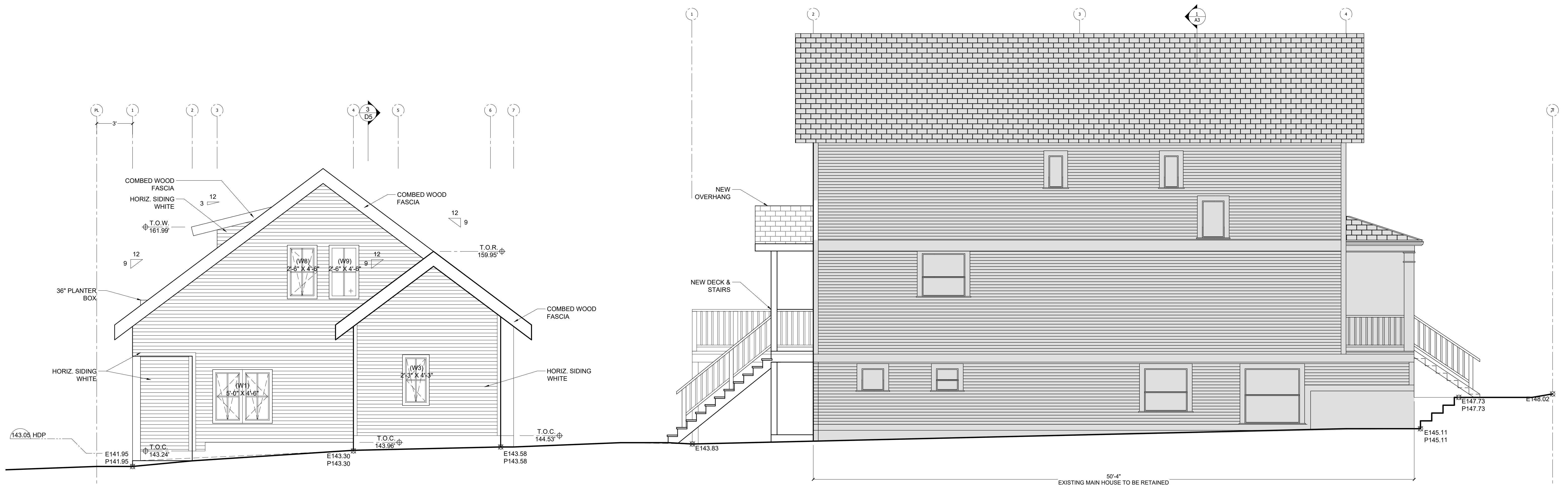
D5.1-4 PROPOSED INFILL & PROPOSED MAIN HOUSE - WEST ELEVATION 1/4" - 1'-0"
