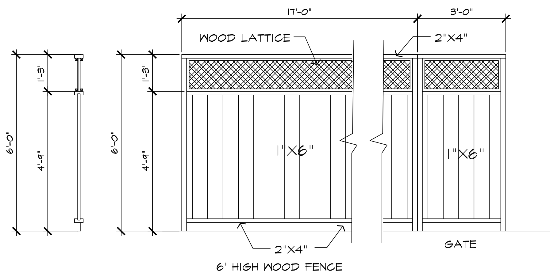
FENCE DETAIL AND SECTION
