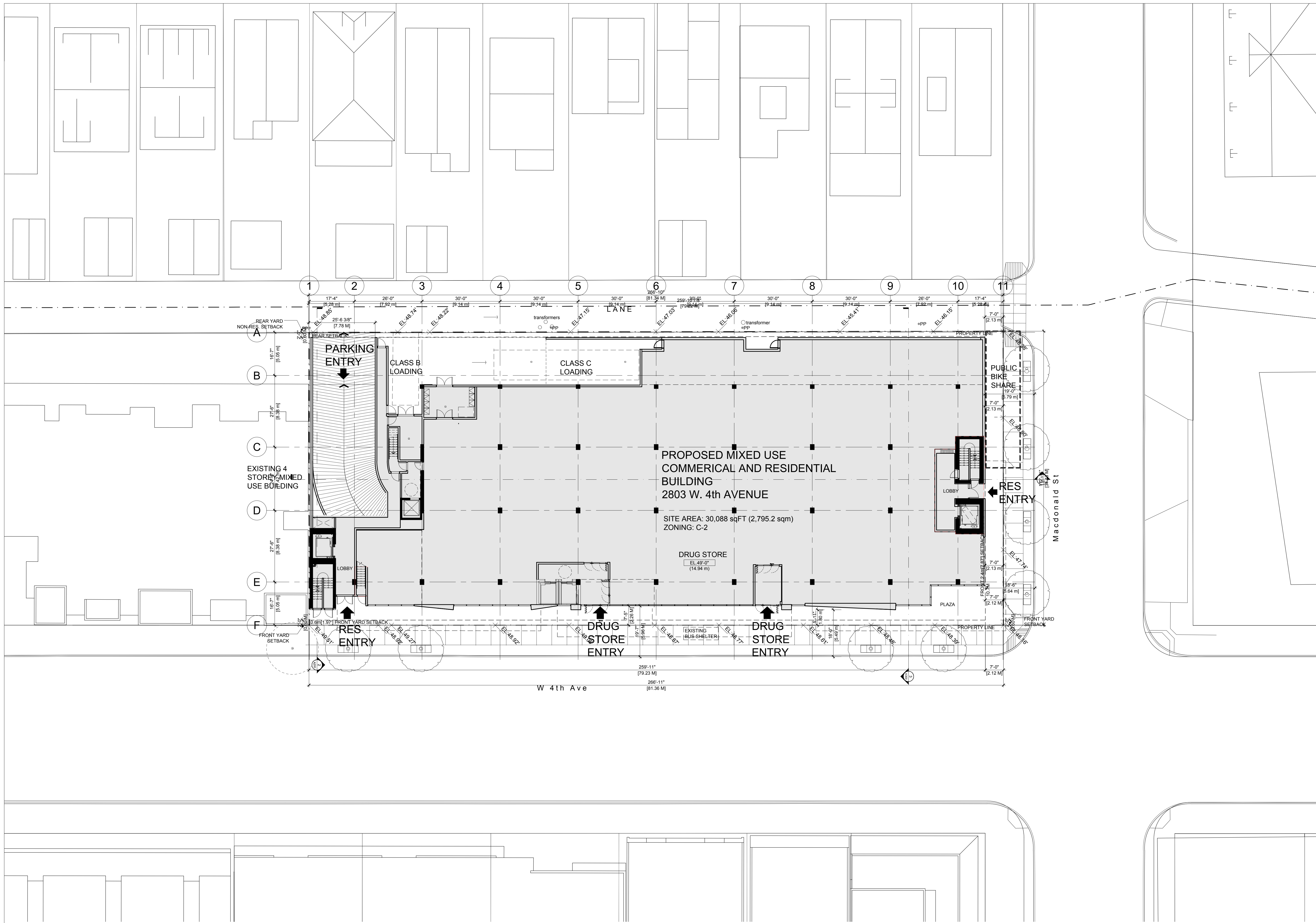
1 SITE PLAN A101 Scale: 1/16"=1'-0"
