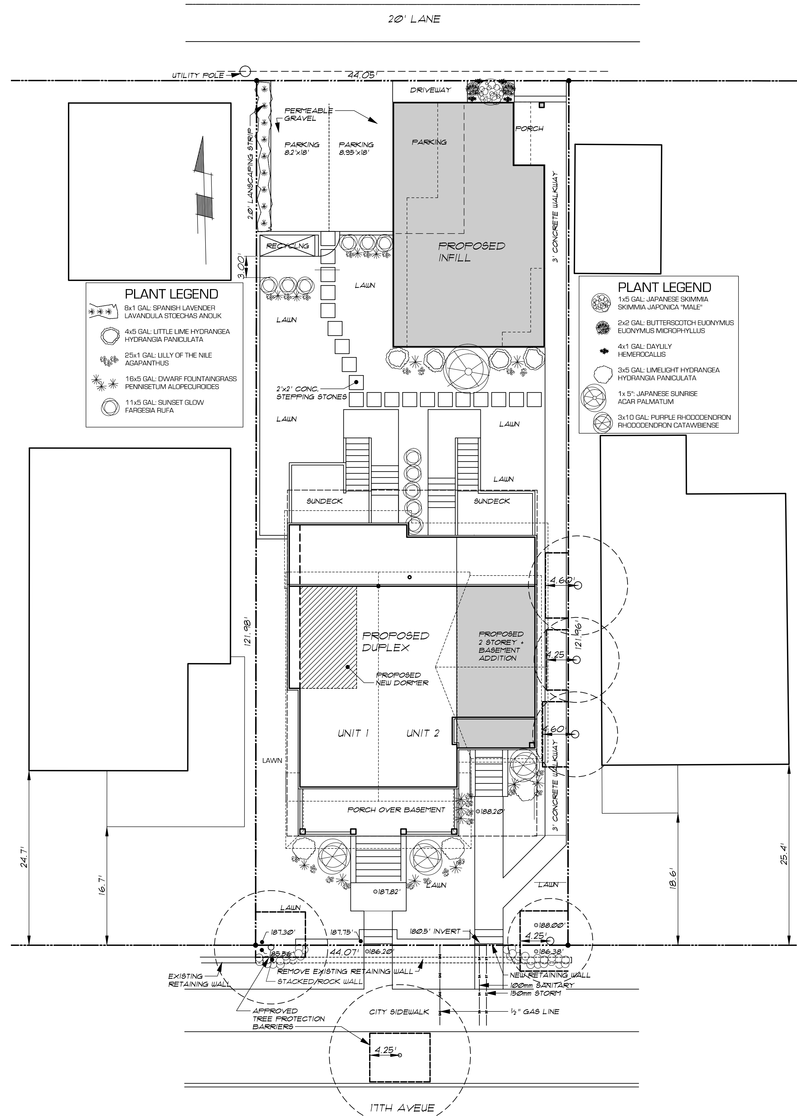
landscape plan scale: 1"=8'
