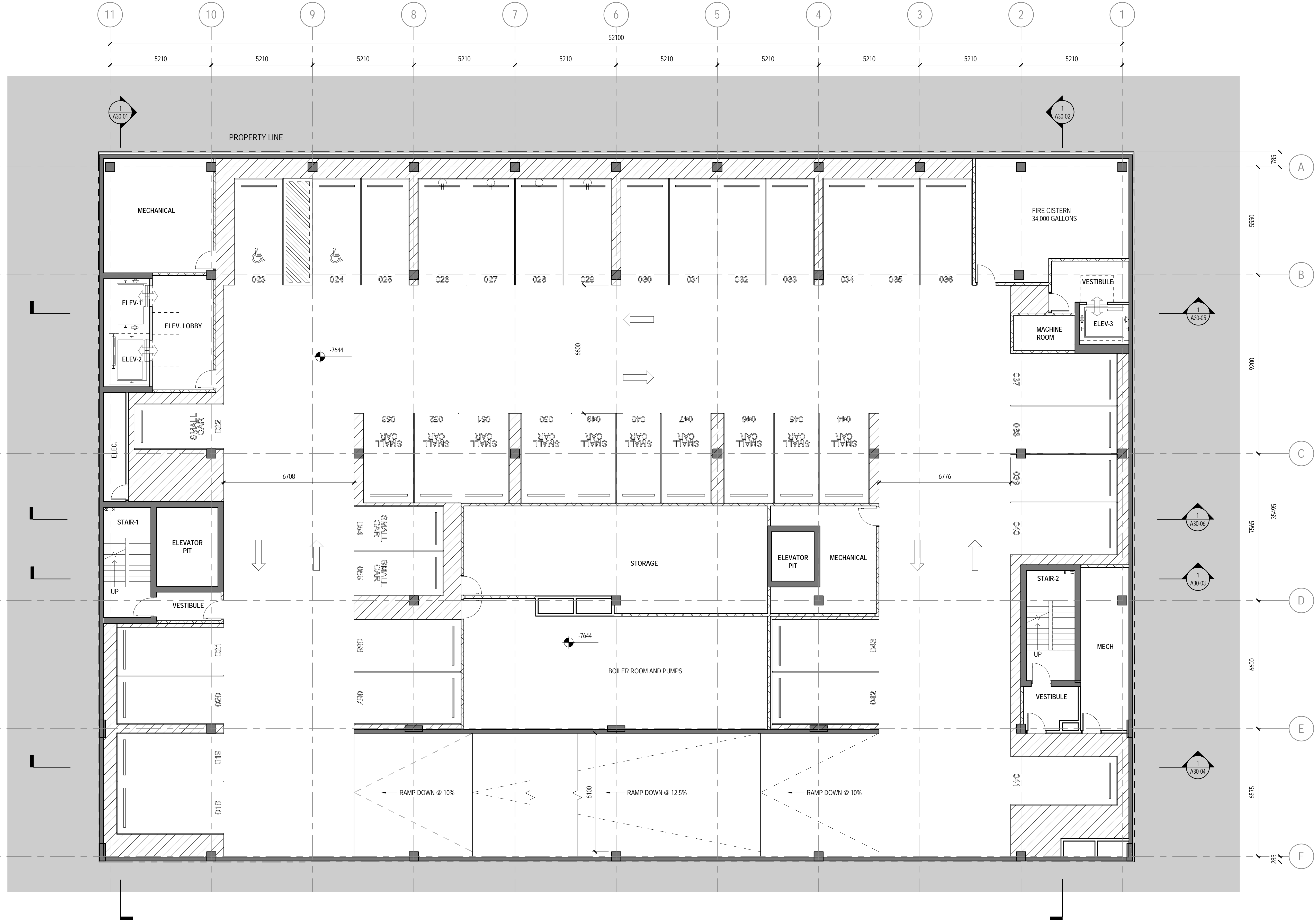
1 LEVEL P2 1:100
