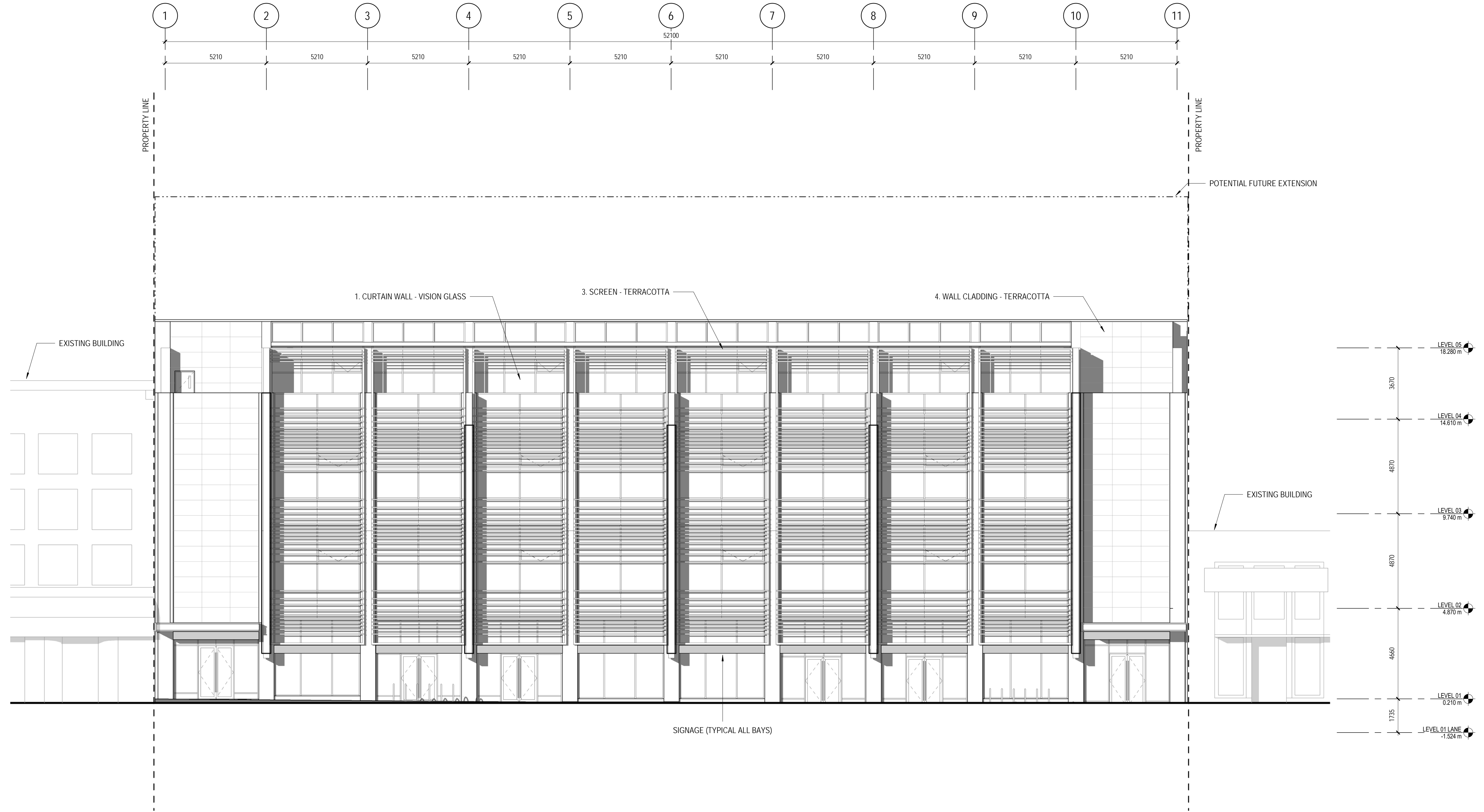
1 NORTH ELEVATION 1 : 100
