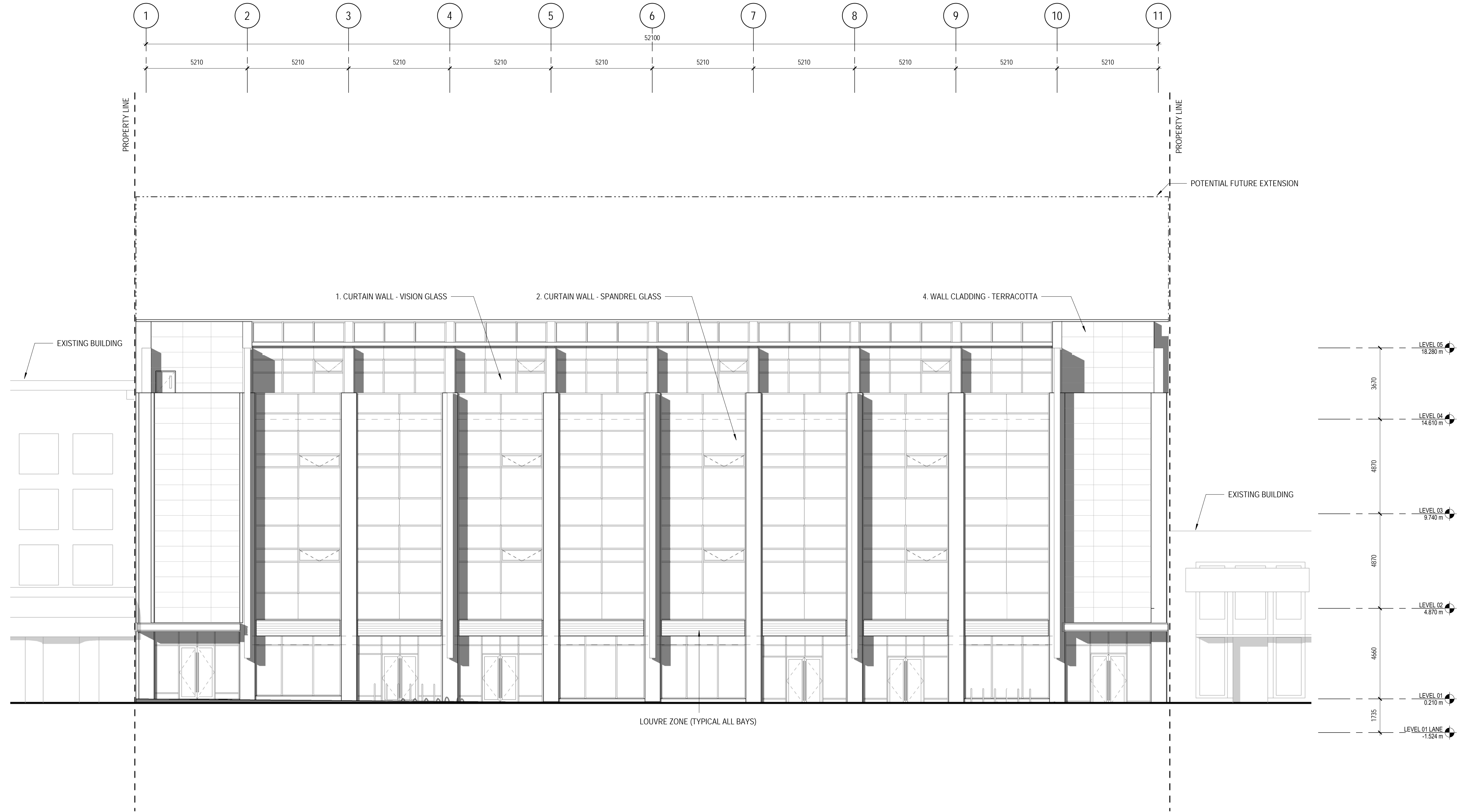
1 NORTH ELEVATION CURTAIN WALL ONLY 1 : 100
