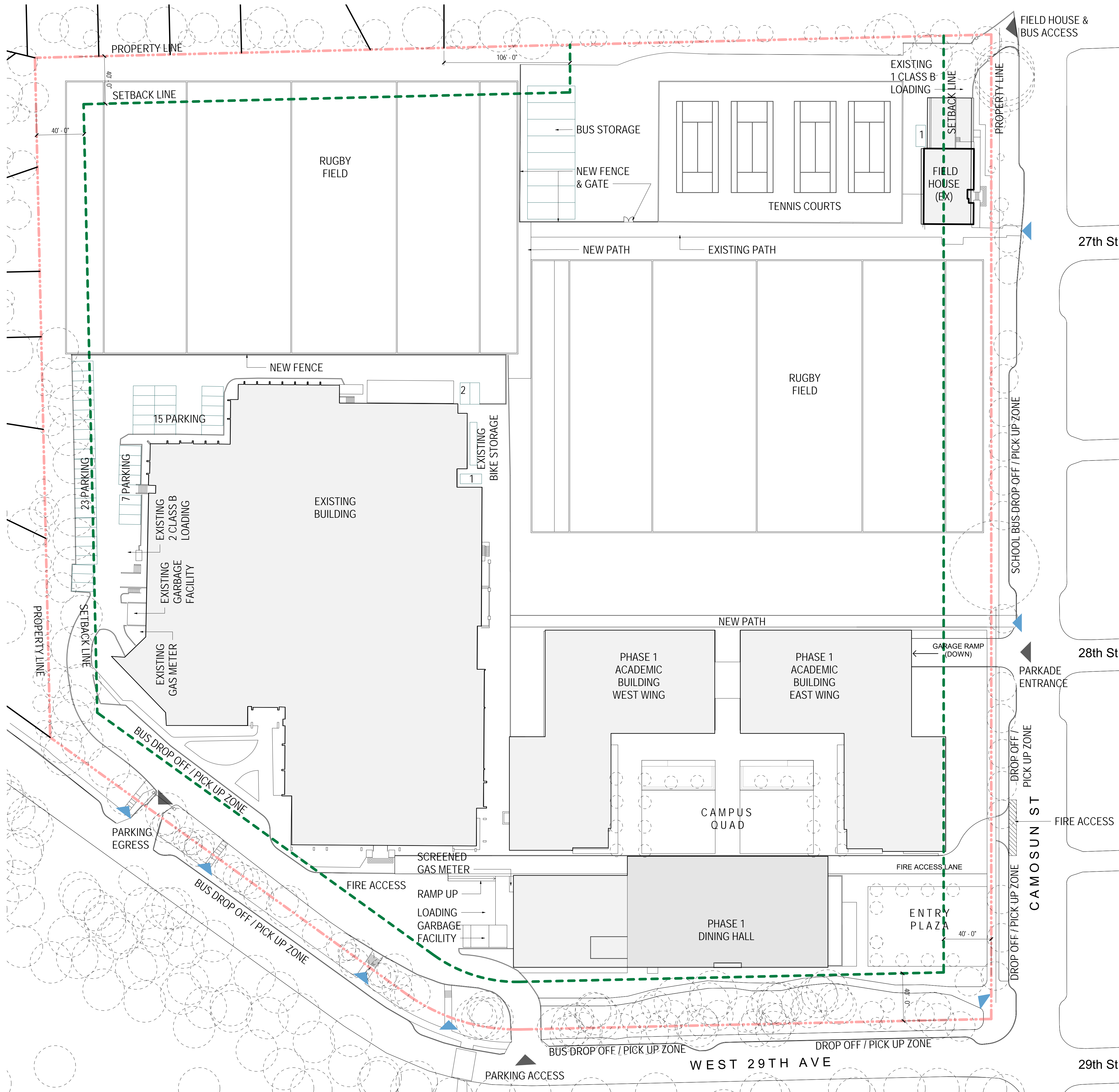
1 SITE PLAN - PHASE ONE SCALE: 1" = 40'-0"
