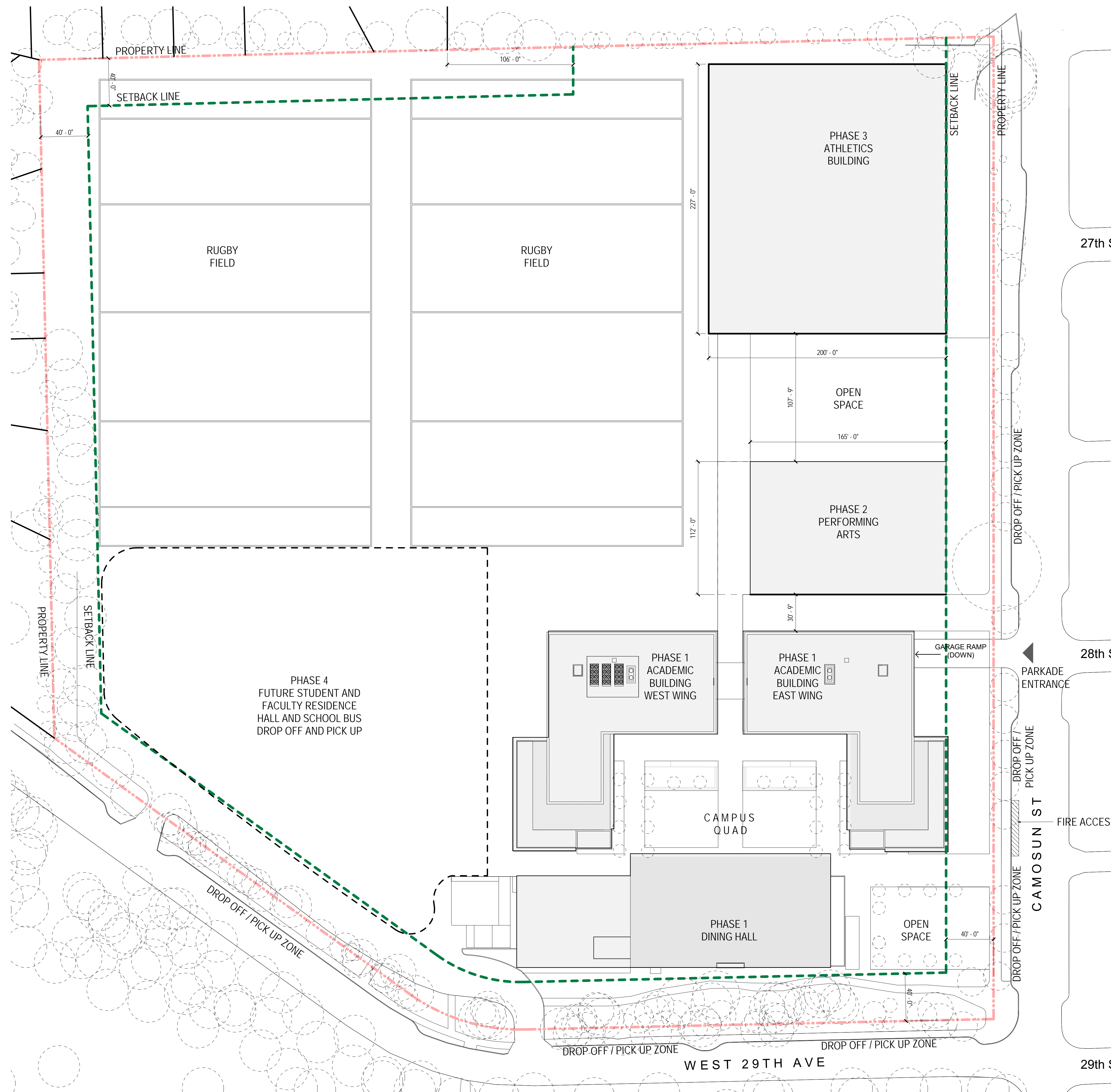
1 SITE PLAN - MASTER PLAN SCALE: 1" = 40'-0"
