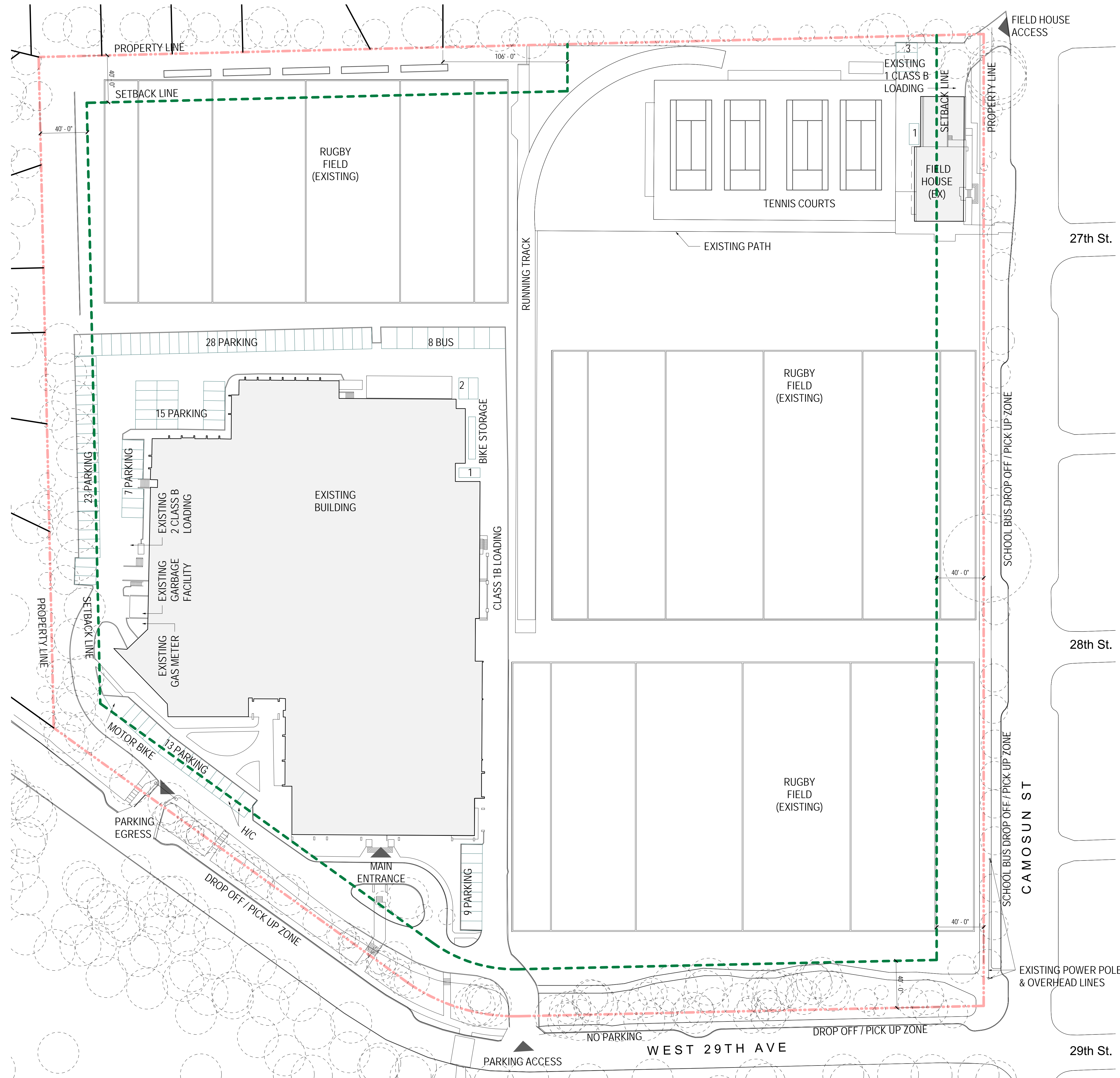
1 SITE PLAN - EXISTING SCALE: 1" = 40'-0"
