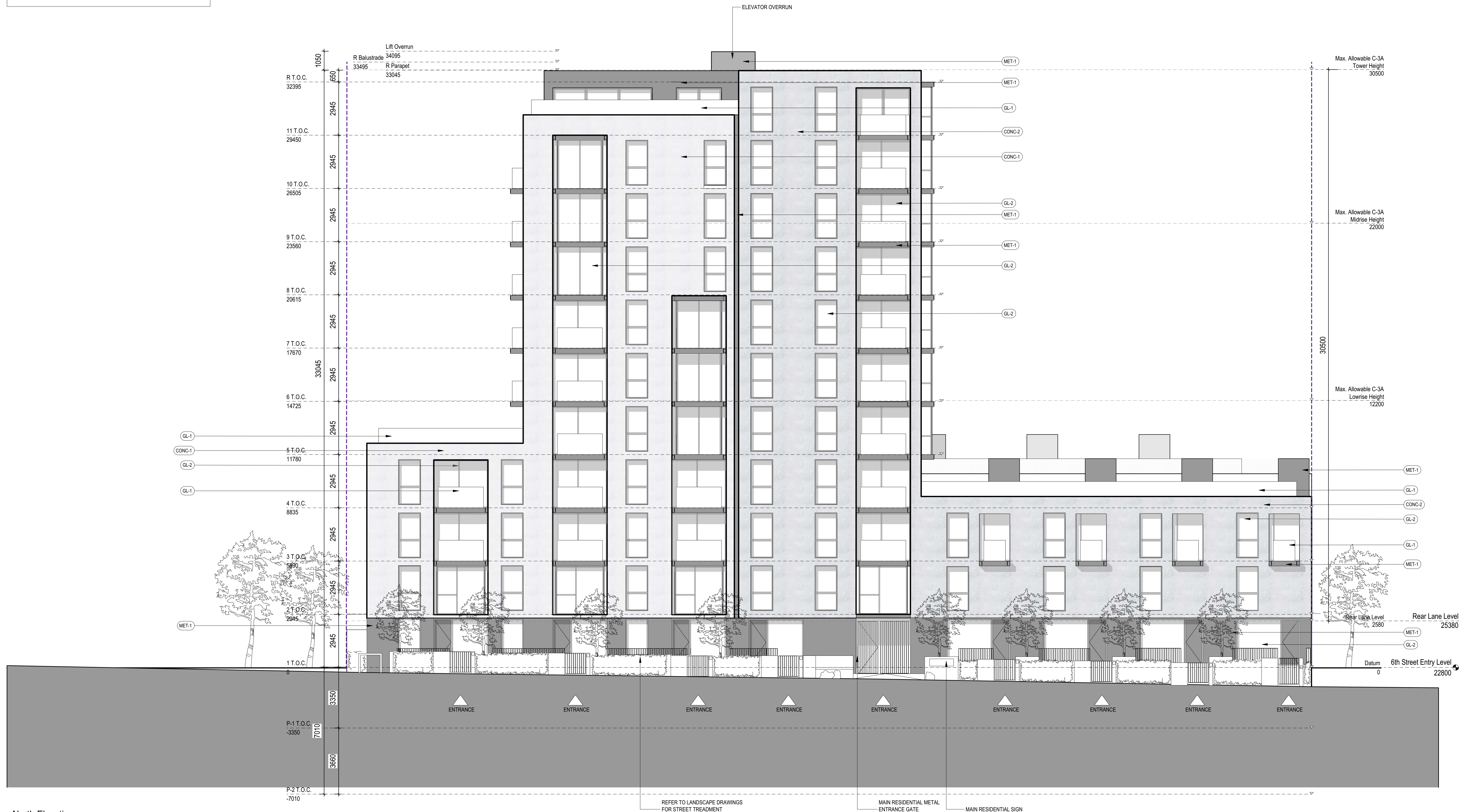
1 North Elevation 1:100
