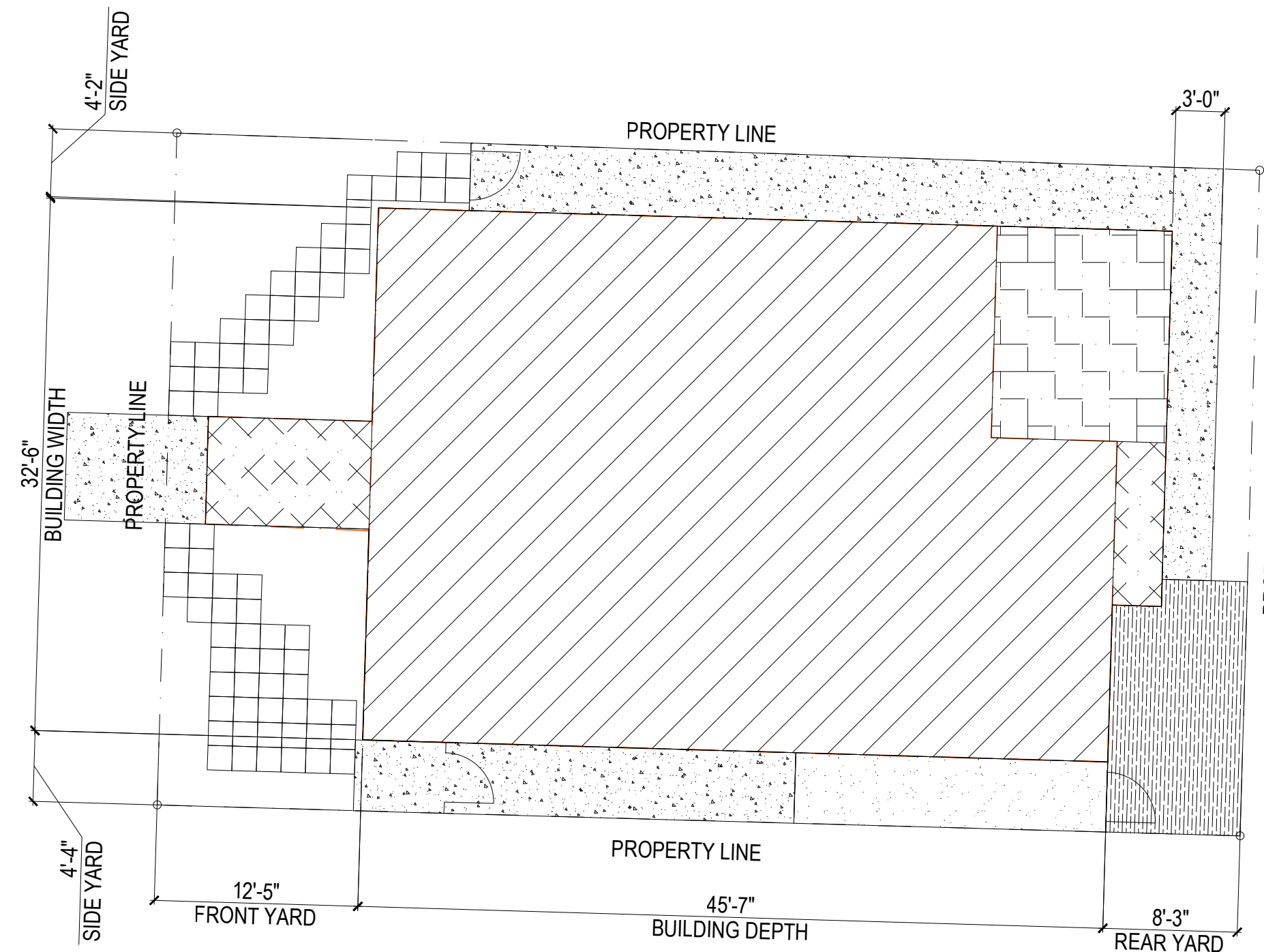
1 SITE COVERAGE AND IMPERMEABLE MATERIAL COVERAGE PLAN SCALE 1/8"= 1'-0"
