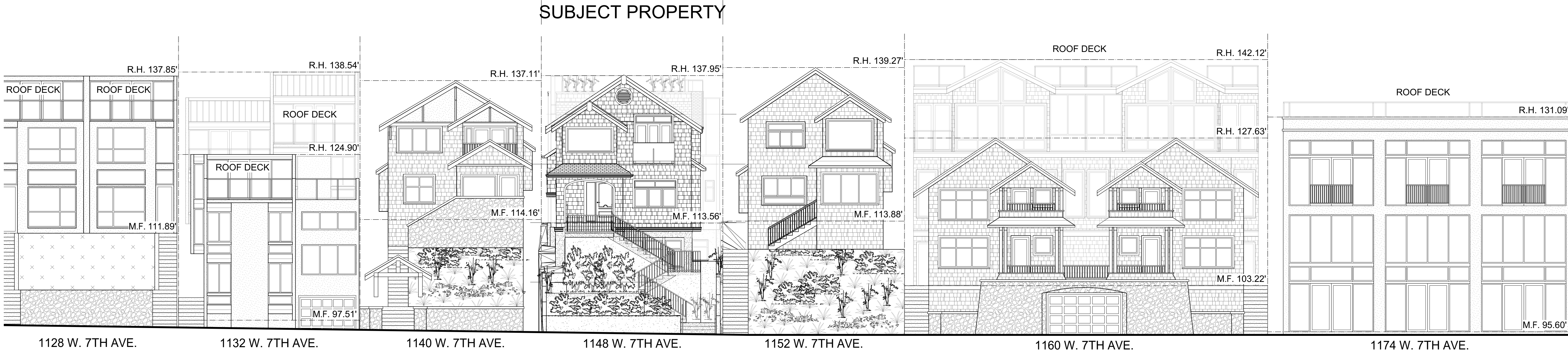
1 STREETFRONT (NORTH) CONTEXT ELEVATION Scale: 1/8" = 1'-0"
