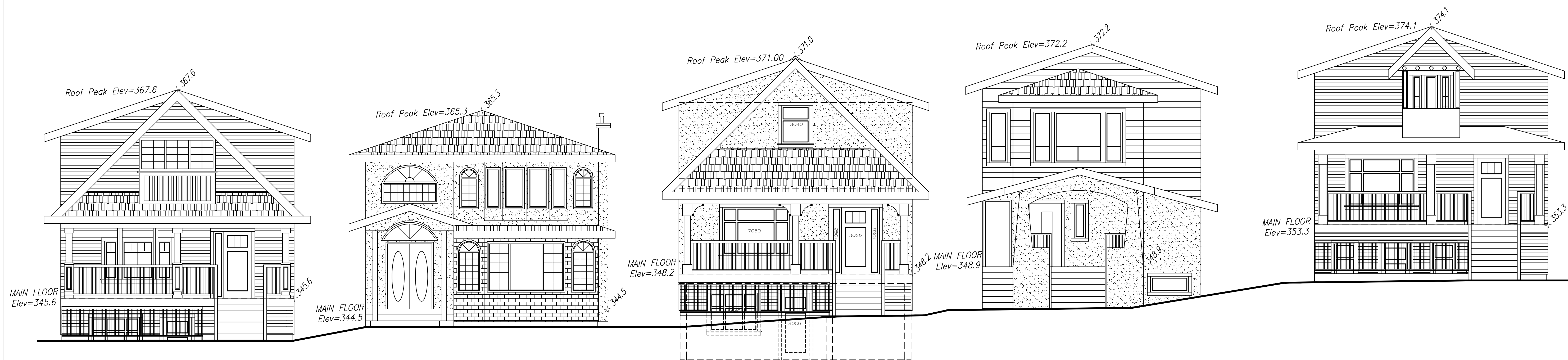
STREET SCAPE SCALE: 3/16" = 1'-0"
