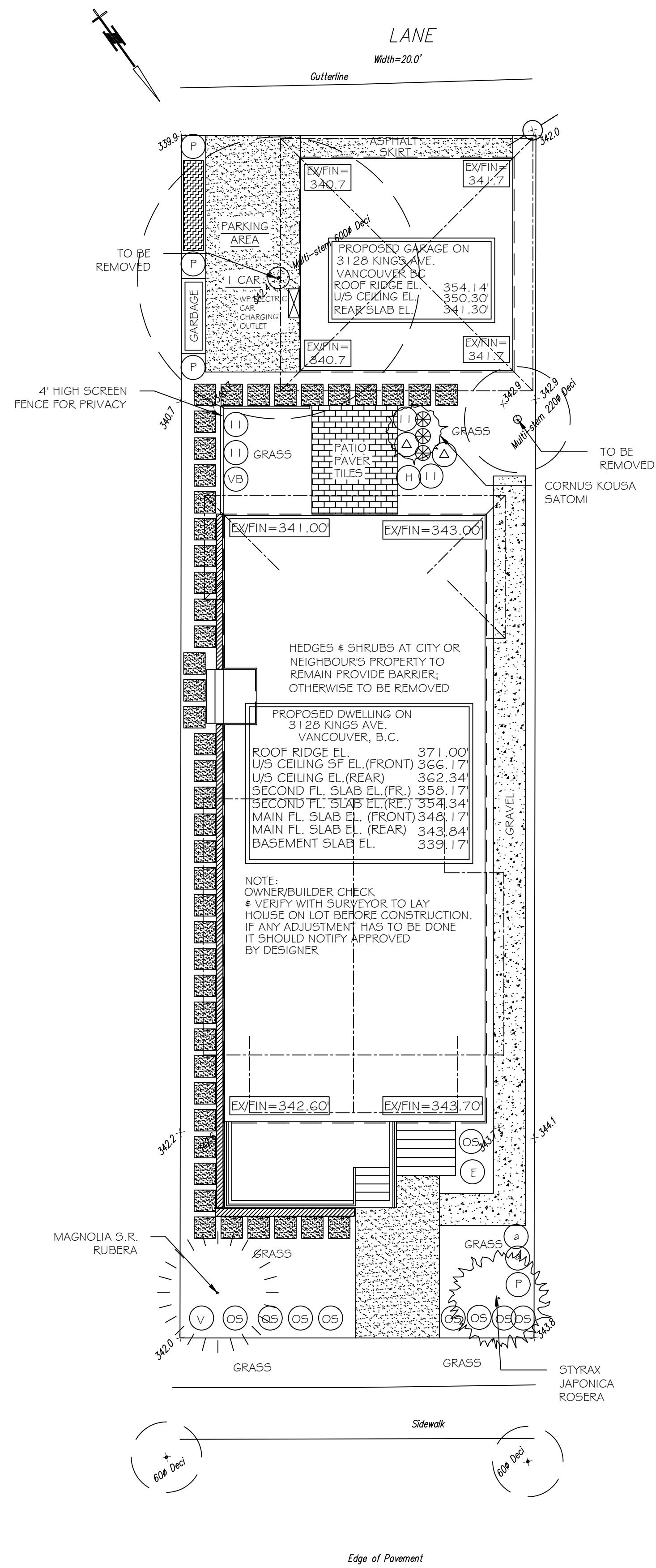
KINGS AVENUE LANDSCAPE PLAN SCALE: 1/8" = 1' - 0"
