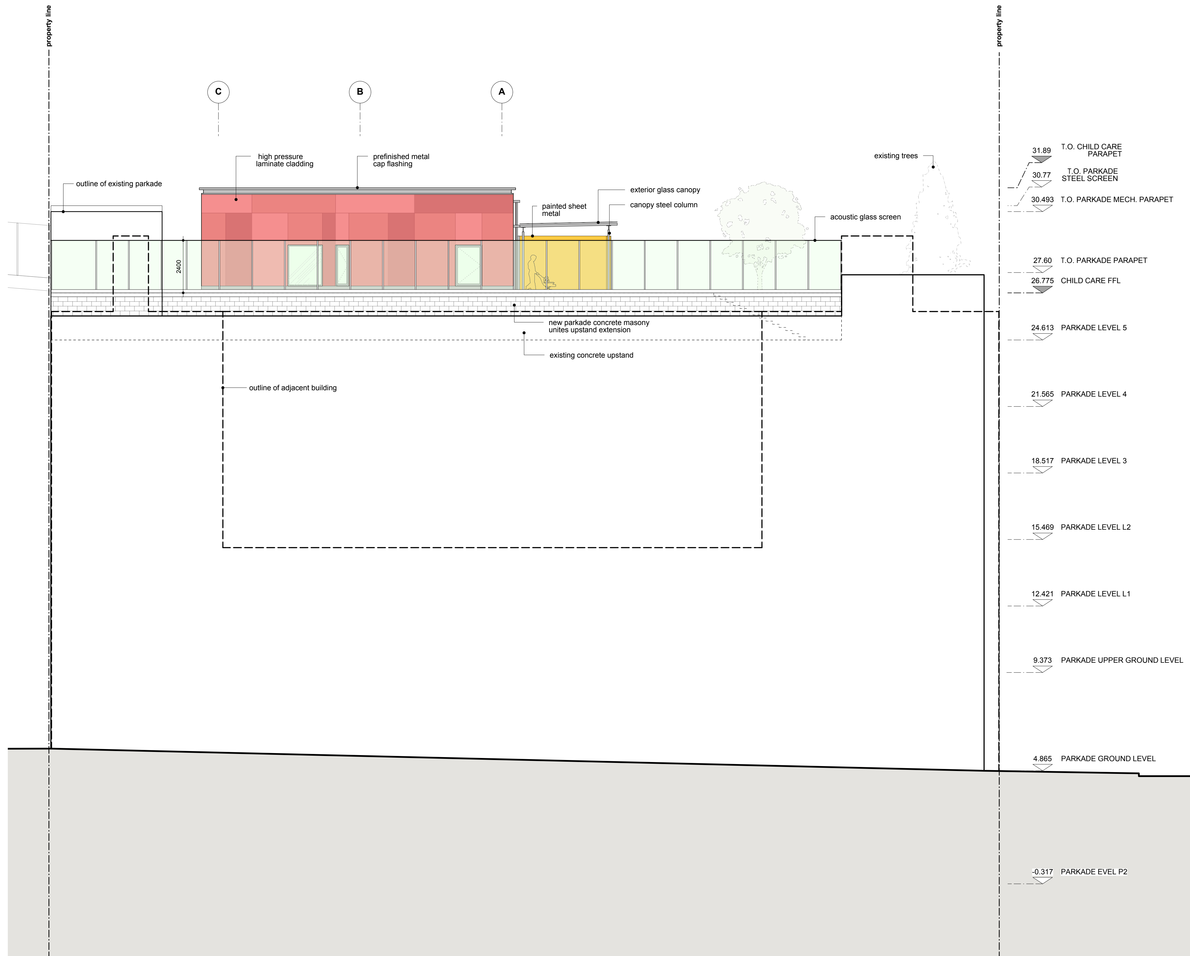
1 water street child care elevation (east)
