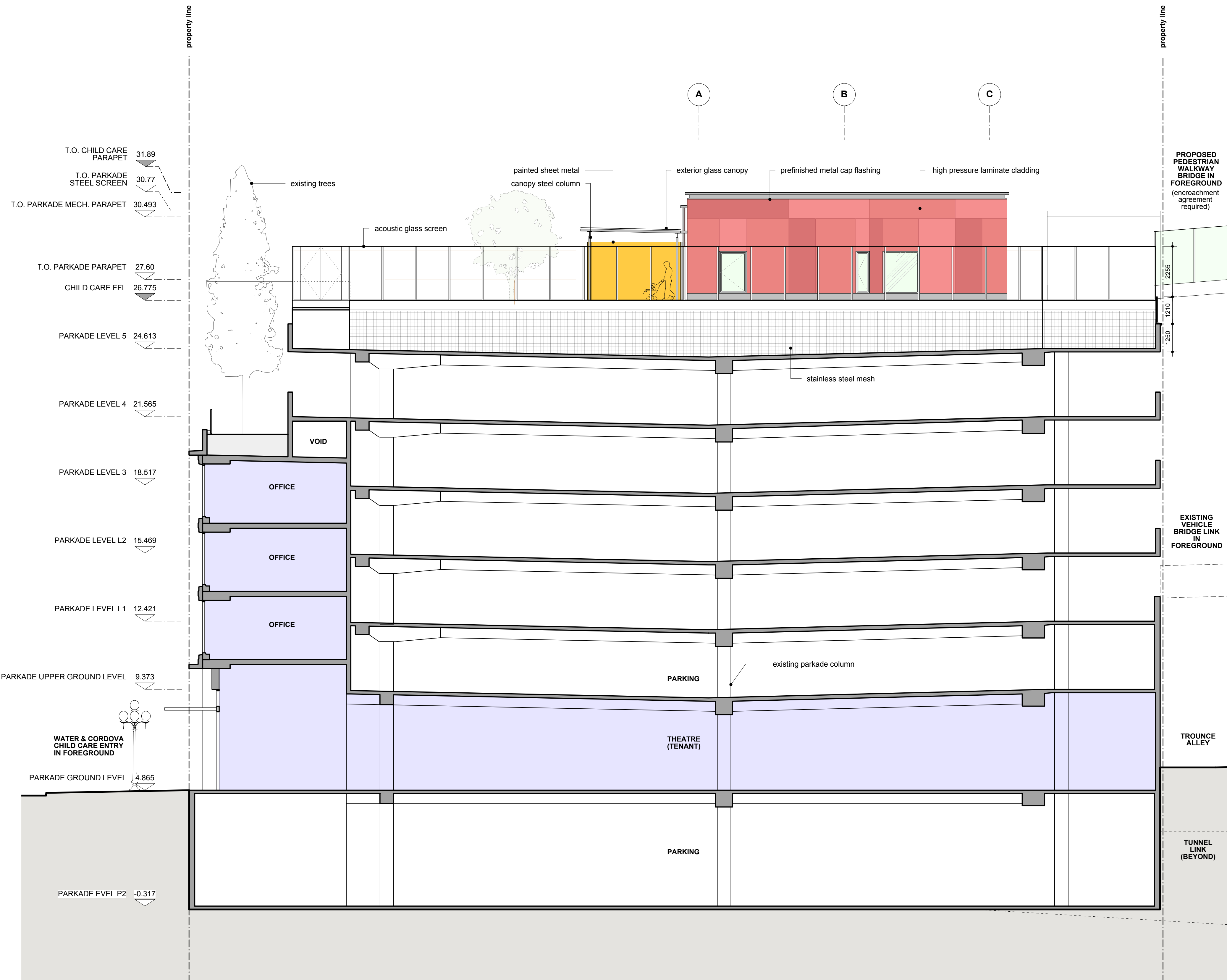
2 water street child care elevation (west)
